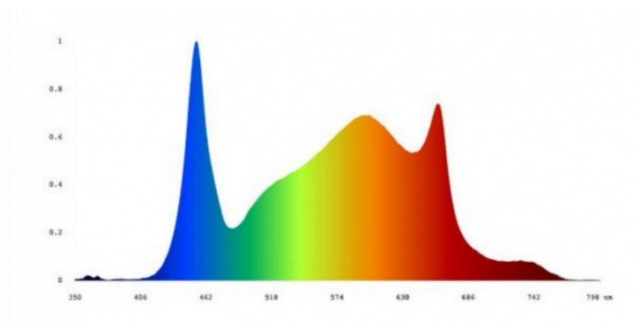
Spectrum
